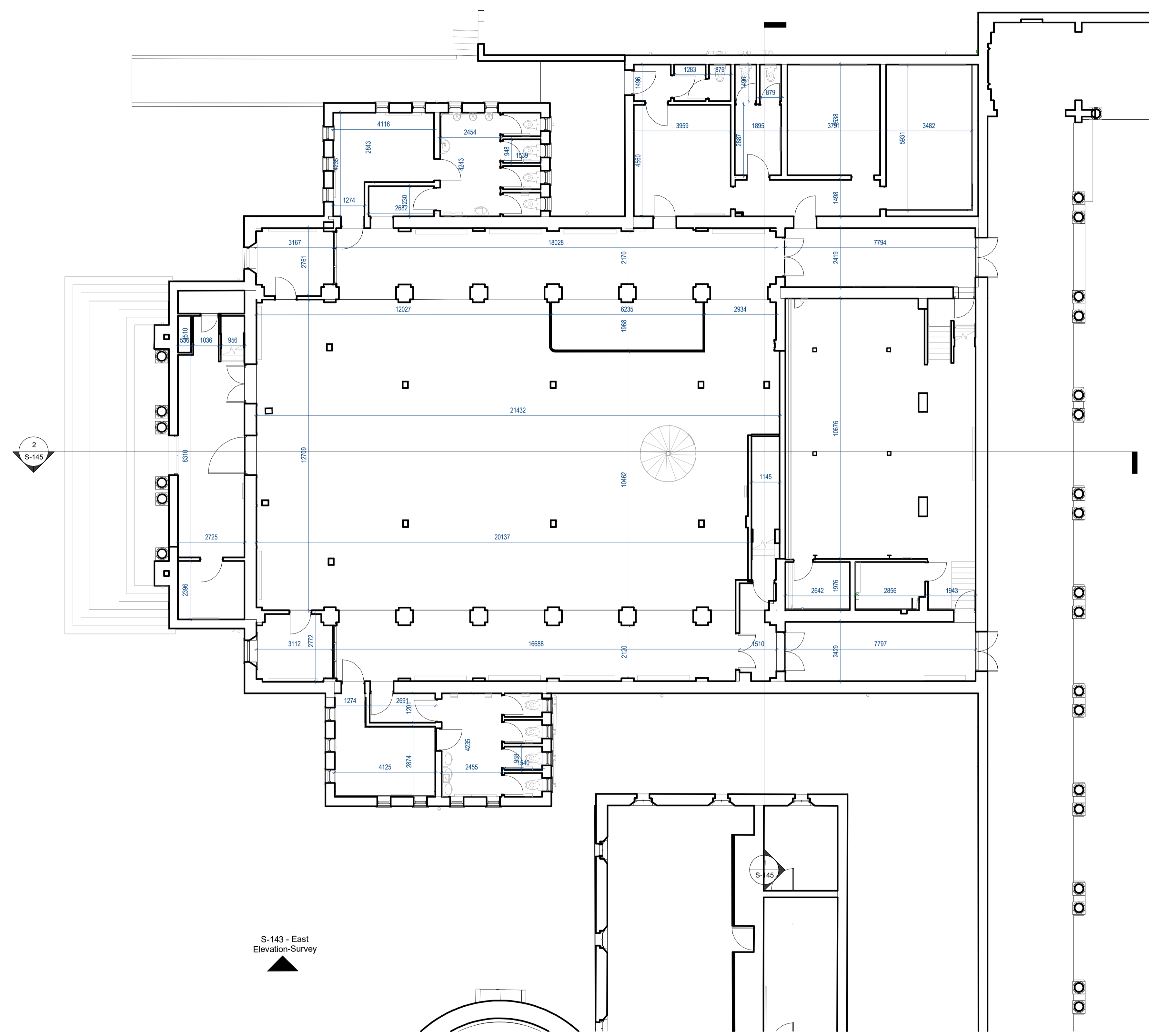
1 Ground Floor-Survey Scale - 1 : 100
